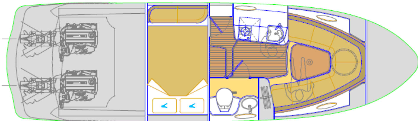
INTERIOR PLAN VIEW.
