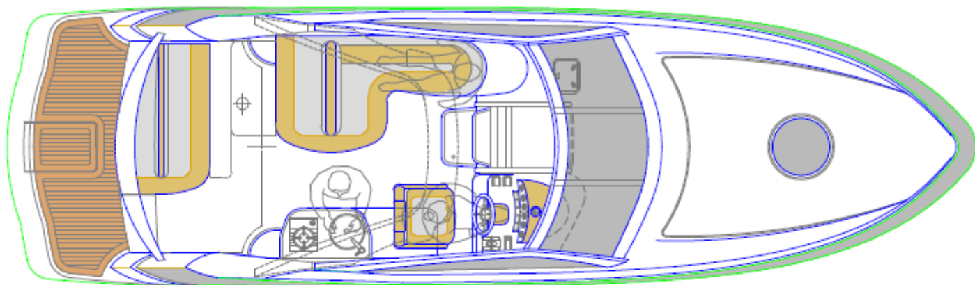
DECK PLAN VIEW.
