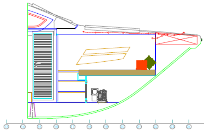
Sectional Viwe
