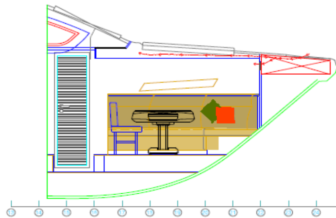
Sectional Viwe
